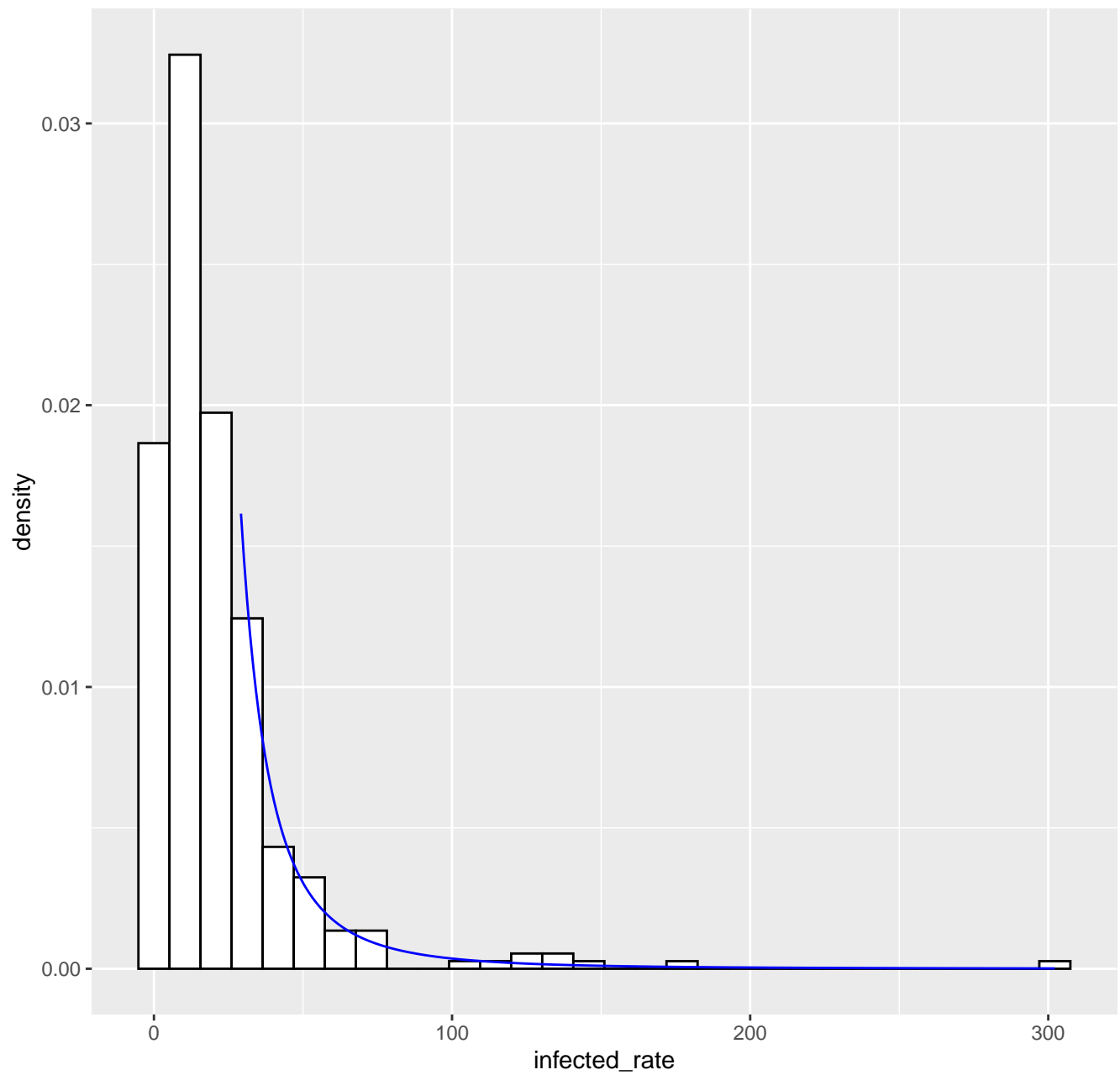
Fitted tail density GPD( 29.2 , 13.95 , 0.49 ), k= 80 -- 21-03-2020
