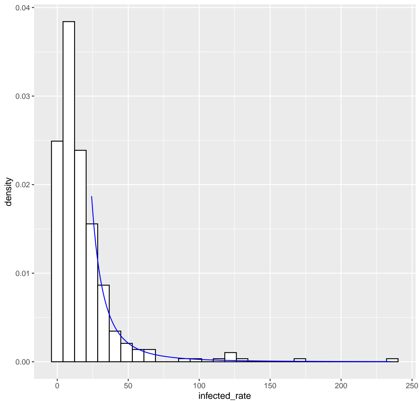
Fitted tail density GPD( 24.2 , 12.05 , 0.51 ), k= 80 -- 20-03-2020
