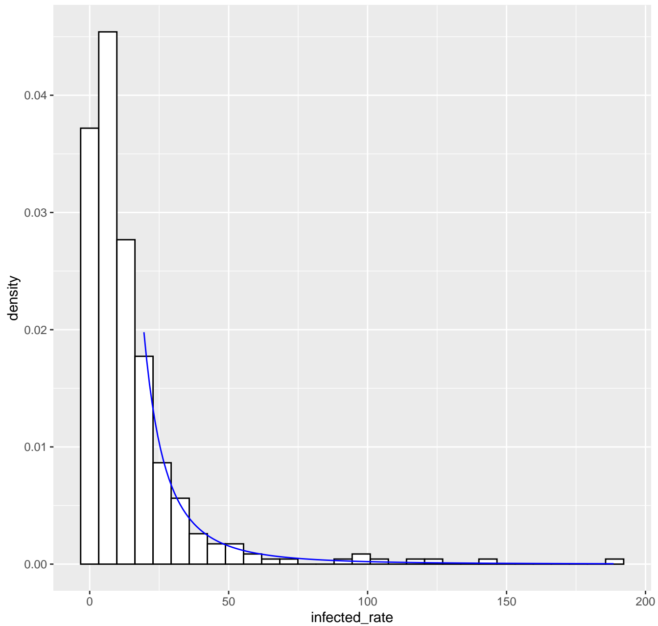
Fitted tail density GPD( 19.51 , 11.39 , 0.5 ), k= 80 -- 19-03-2020
