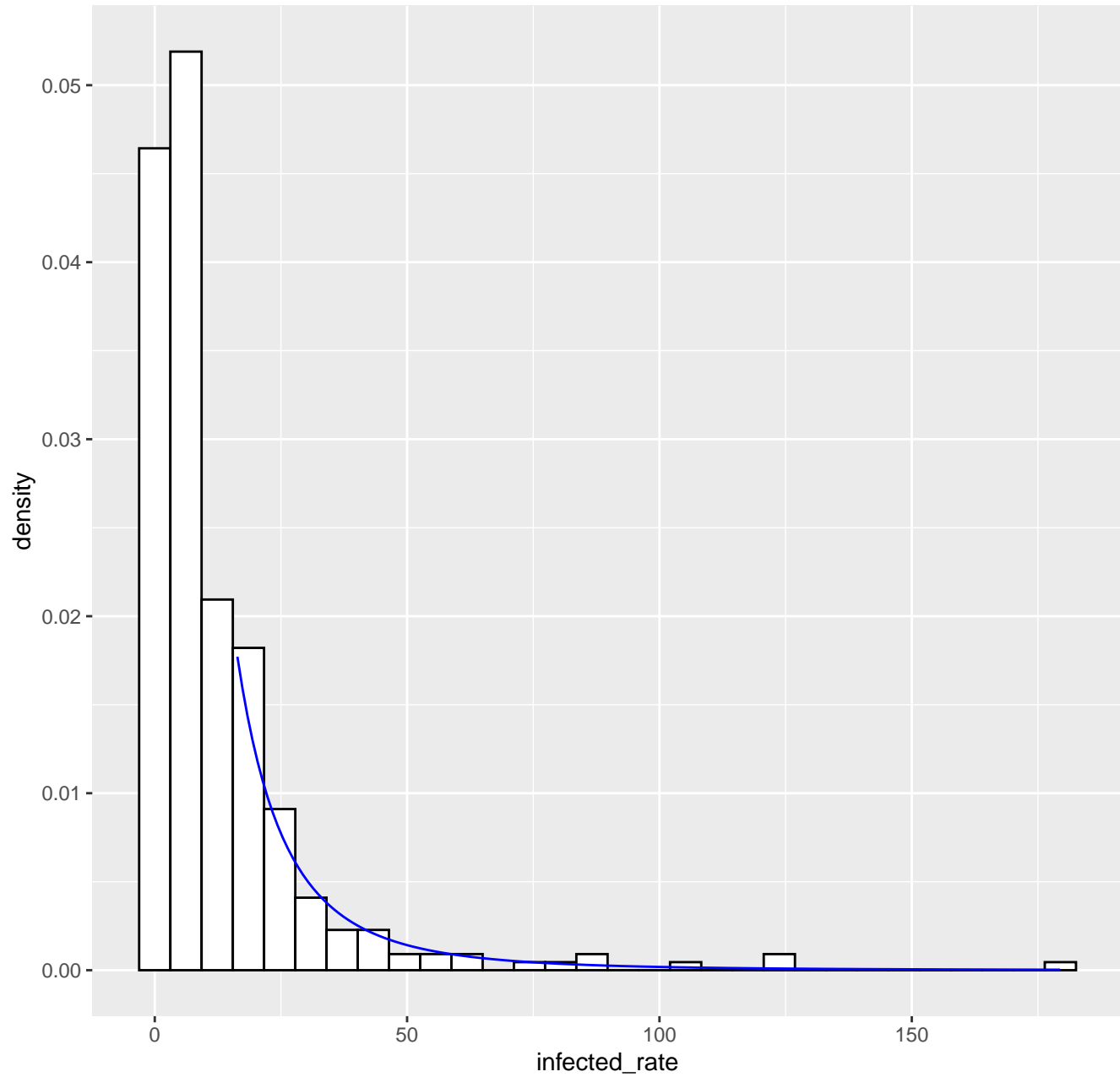
Fitted tail density GPD( 16.38 , 12.72 , 0.37 ), k= 80 -- 18-03-2020
