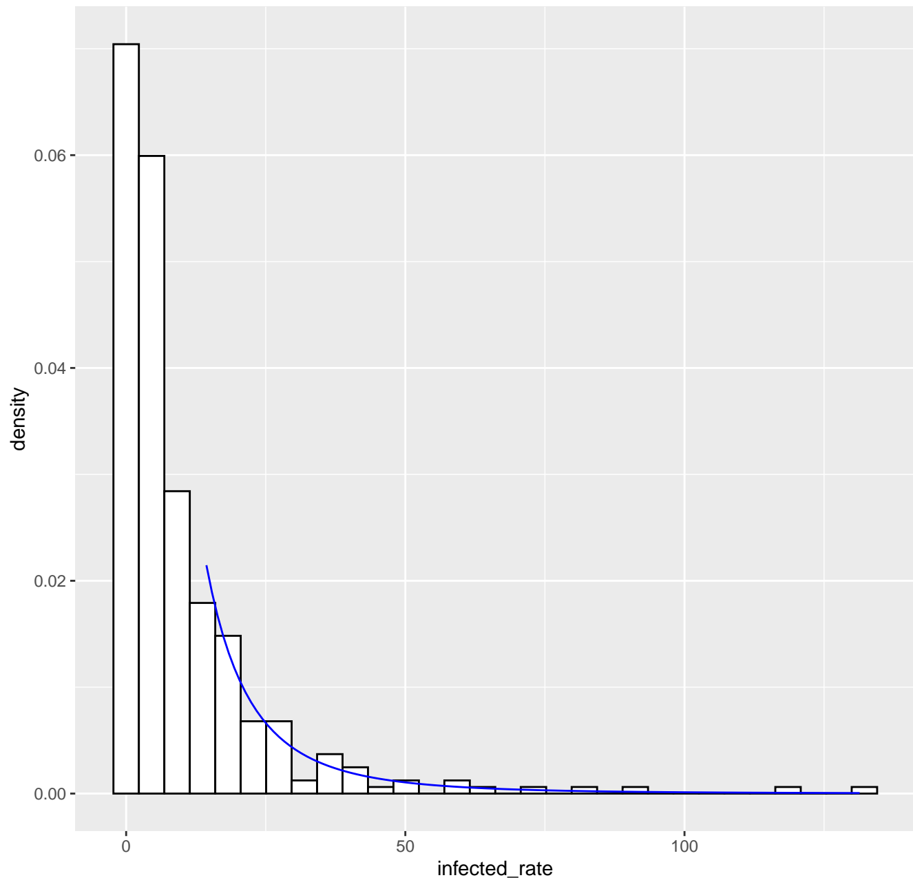
Fitted tail density GPD( 14.37 , 10.5 , 0.36 ), k= 80 -- 17-03-2020
