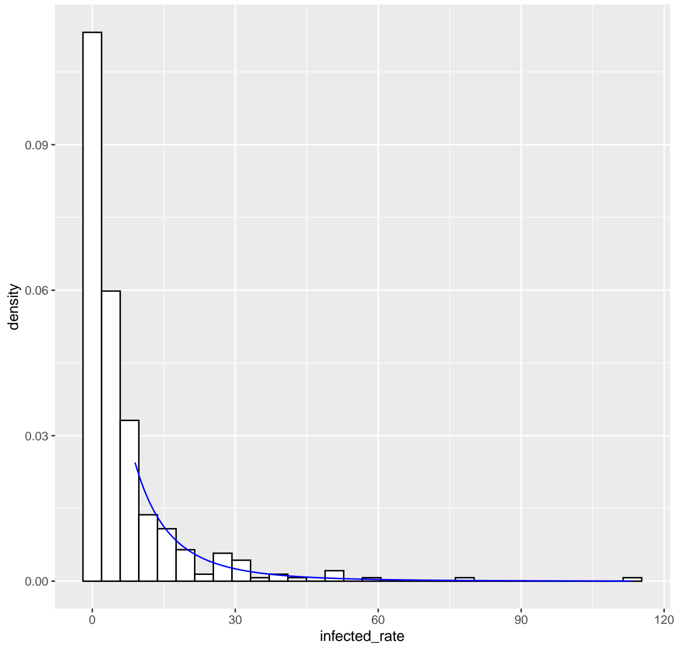
Fitted tail density GPD( 8.96 , 9.21 , 0.29 ), k= 80 -- 15-03-2020
