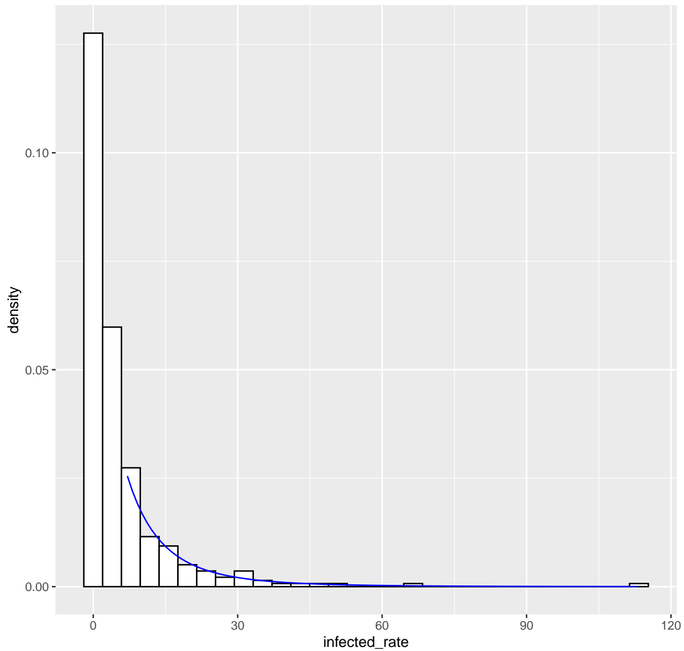
Fitted tail density GPD( 7.09 , 8.84 , 0.25 ), k= 80 -- 14-03-2020
