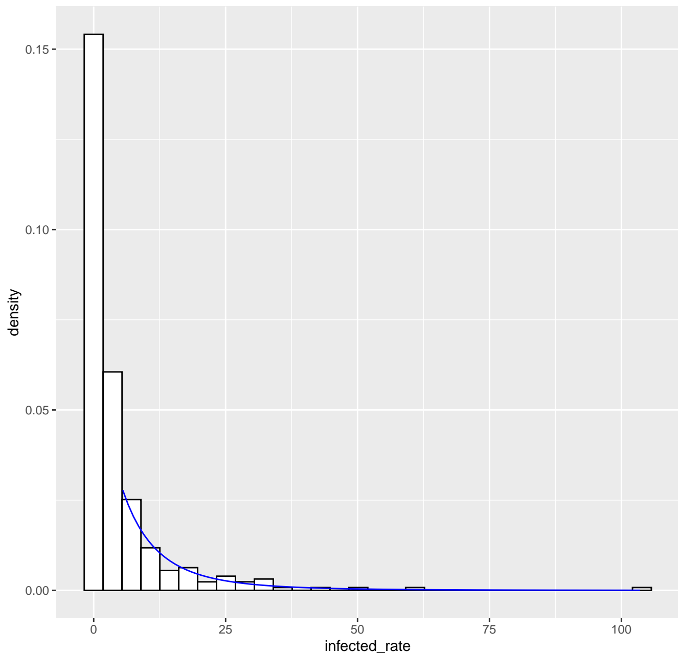
Fitted tail density GPD( 5.52 , 8.12 , 0.27 ), k= 80 -- 13-03-2020
