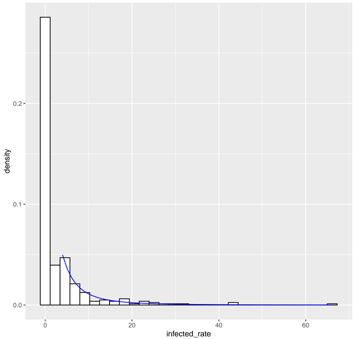
Fitted tail density GPD( 4.01 , 4.54 , 0.46 ), k= 80 -- 11-03-2020
