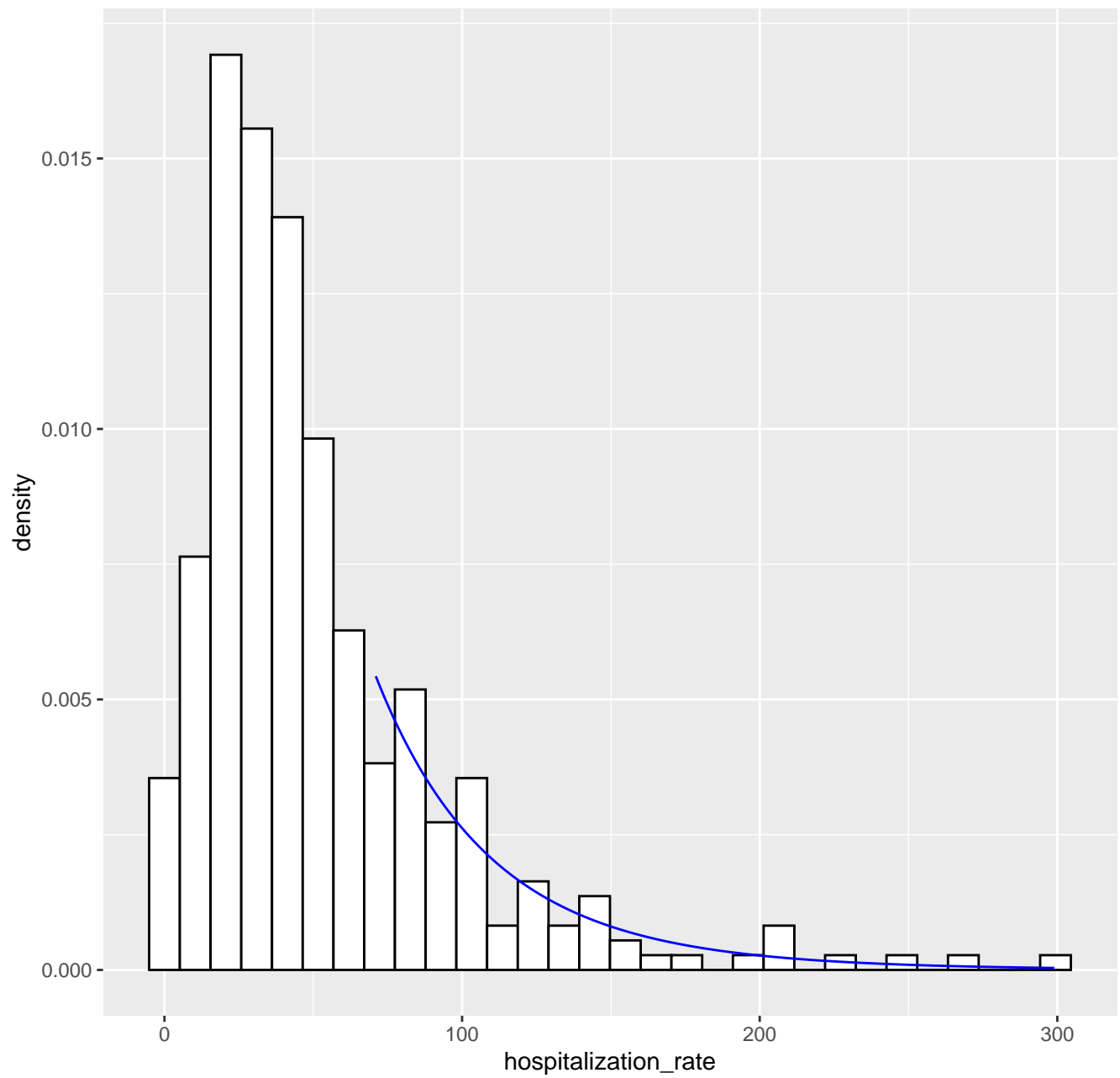
Fitted tail density GPD( 71 , 41.51 , 0.07 ), k= 80 -- 10-04-2020
