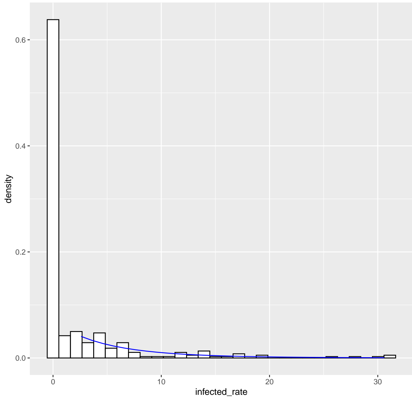
Fitted tail density GPD( 2.59 , 5.54 , 0.12 ), k= 80 -- 10-03-2020
