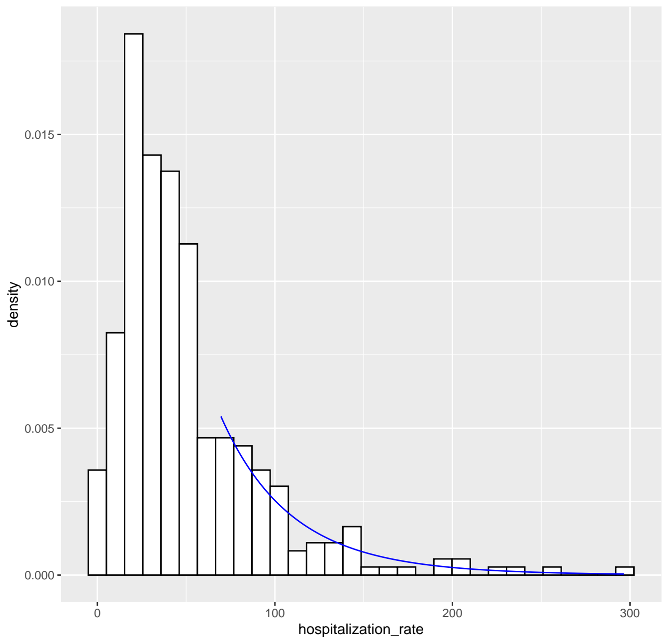
Fitted tail density GPD( 69.6 , 41.72 , 0.06 ), k= 80 -- 09-04-2020
