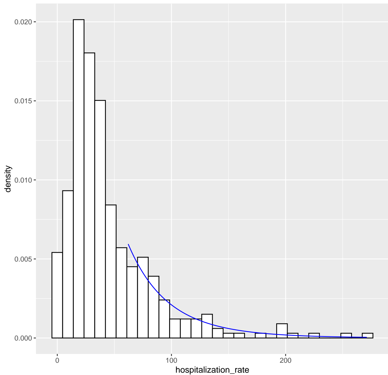
Fitted tail density GPD( 62.1 , 37.92 , 0.09 ), k= 80 -- 06-04-2020
