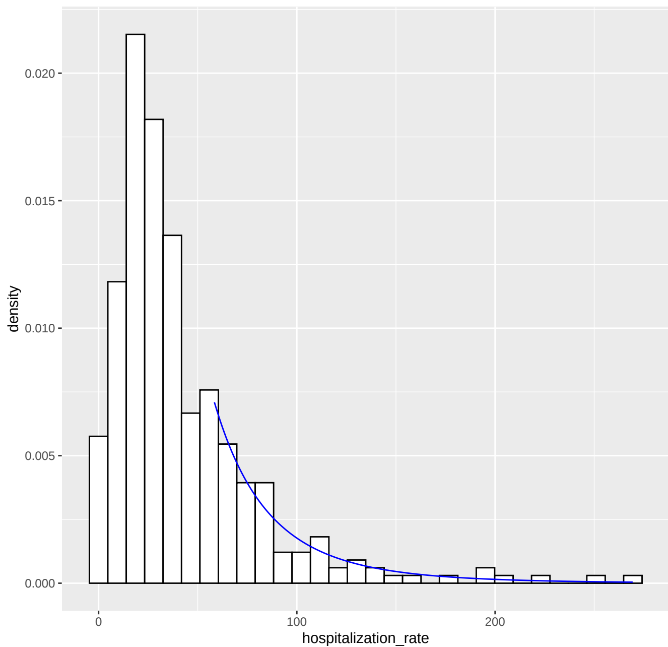
Fitted tail density GPD( 58.4 , 31.76 , 0.18 ), k= 80 -- 04-04-2020
