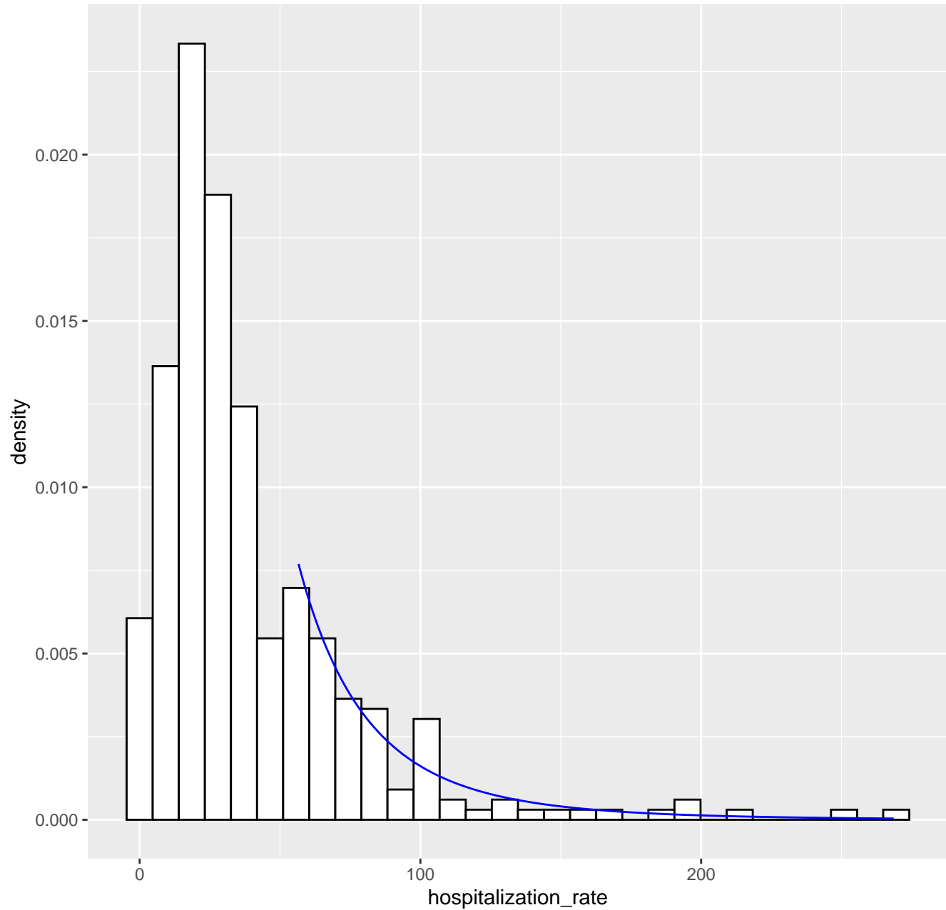
Fitted tail density GPD( 56.6 , 29.3 , 0.21 ), k= 80 -- 03-04-2020
