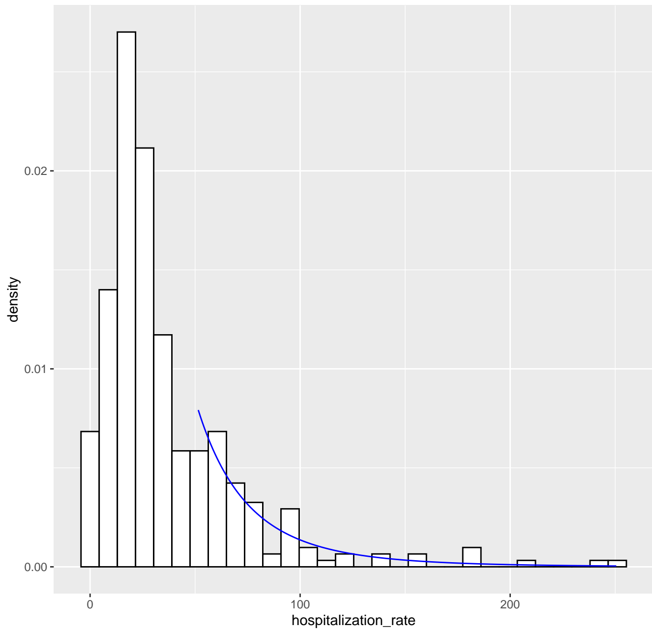
Fitted tail density GPD( 51.5 , 28.45 , 0.21 ), k= 80 -- 02-04-2020
