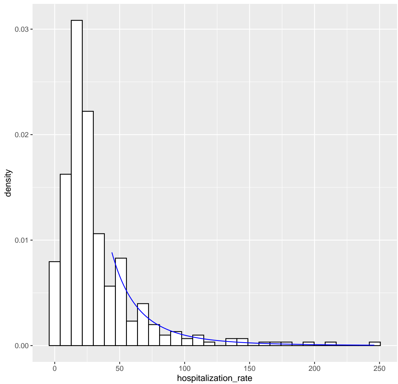
Fitted tail density GPD( 44 , 25.5 , 0.28 ), k= 80 -- 01-04-2020
