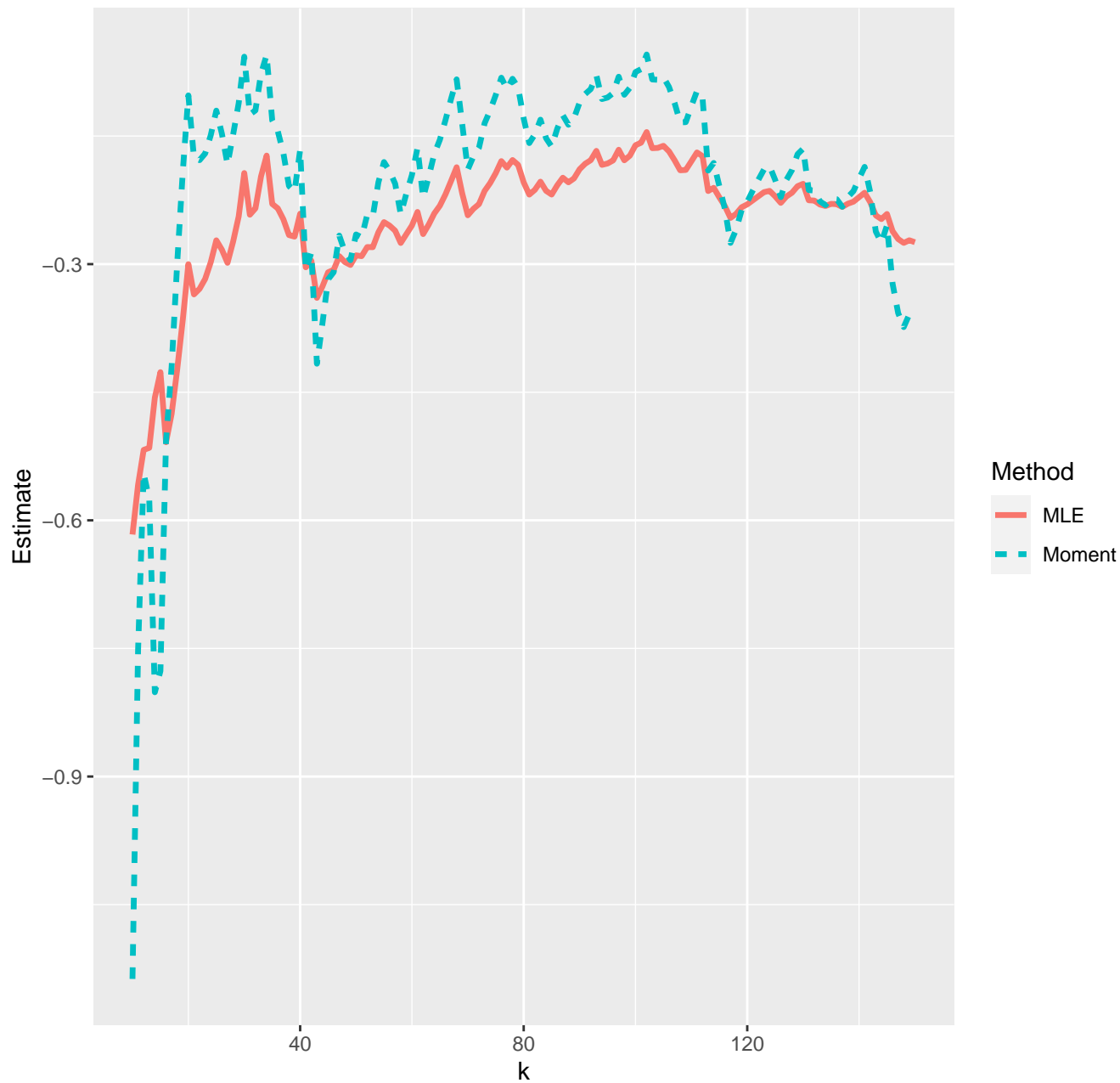
Estimates of extreme value index--31-08-2021
