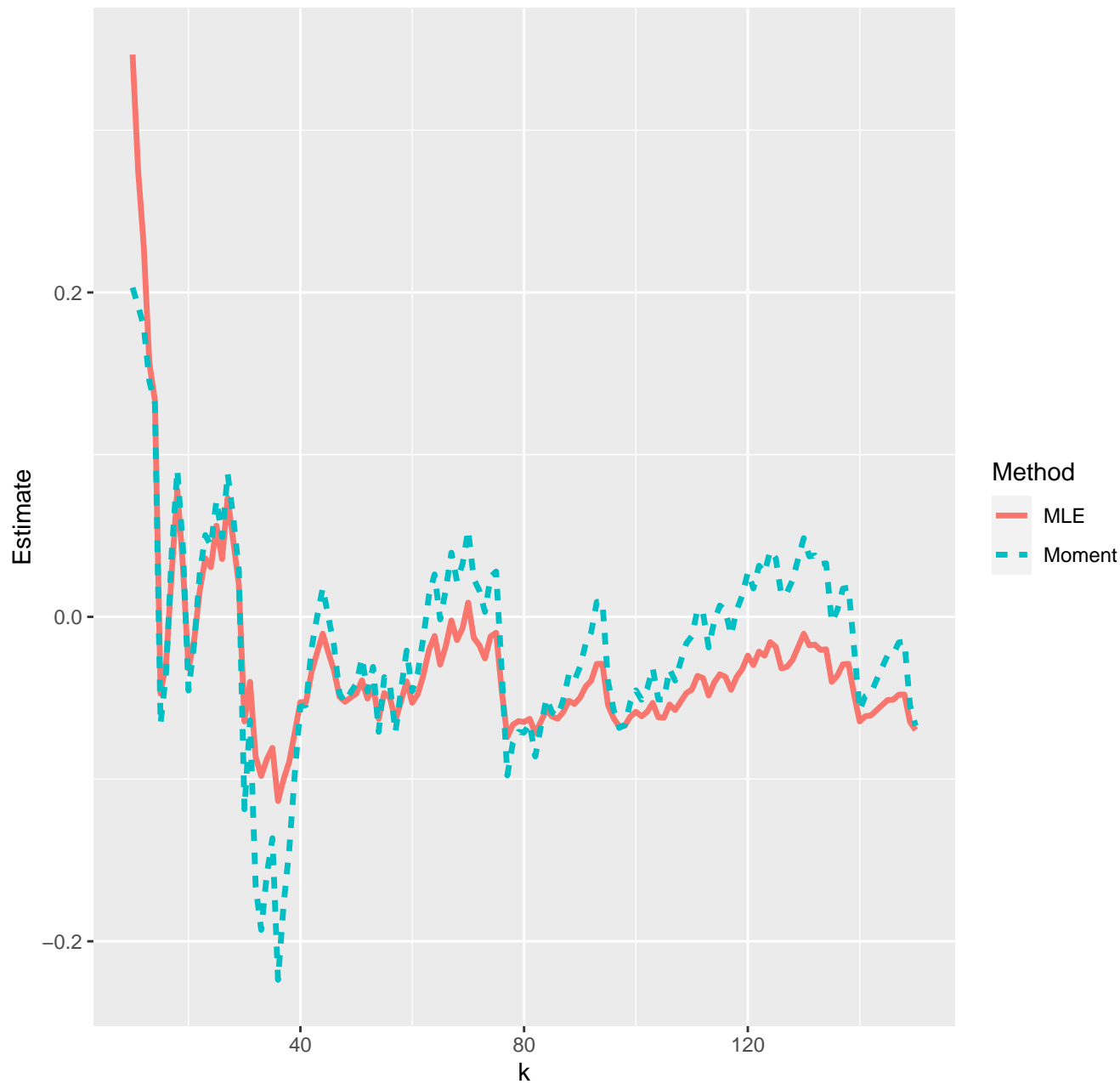
Estimates of extreme value index--31-05-2022
