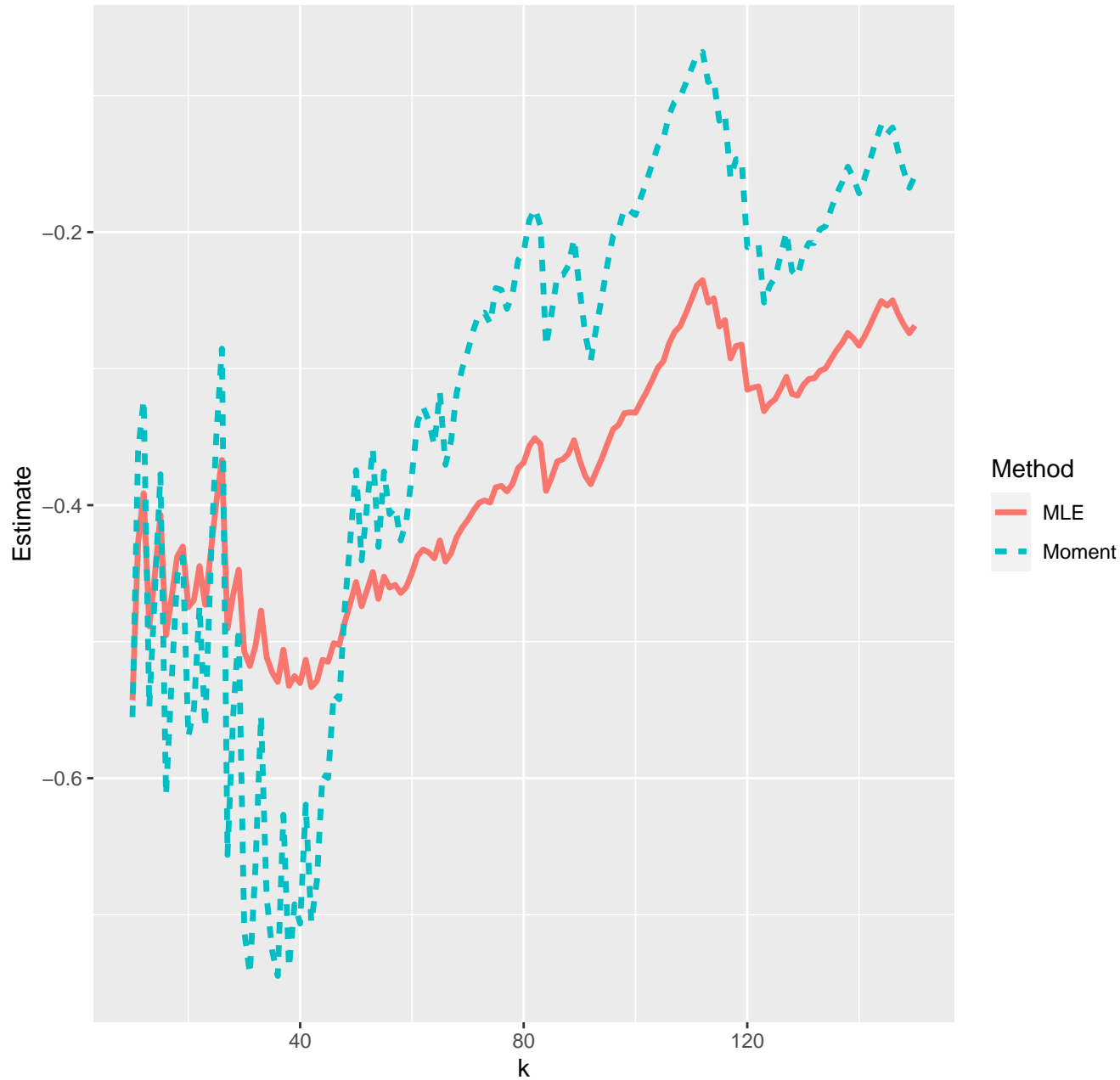
Estimates of extreme value index--30-11-2021
