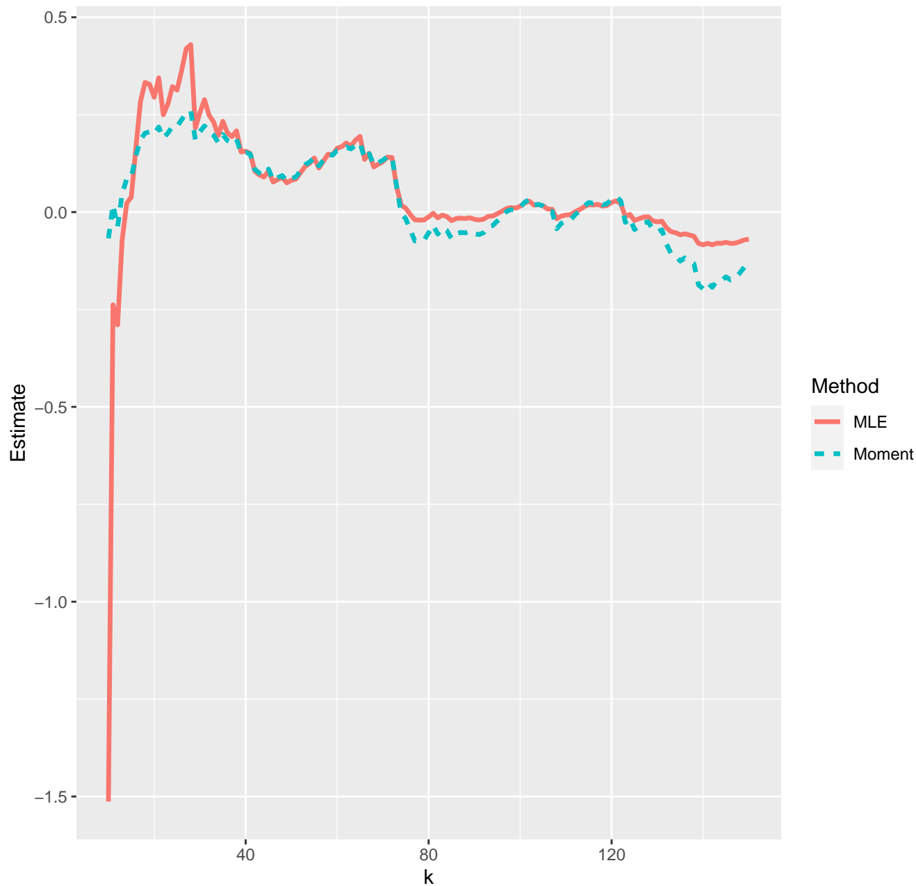
Estimates of extreme value index--30-03-2021
