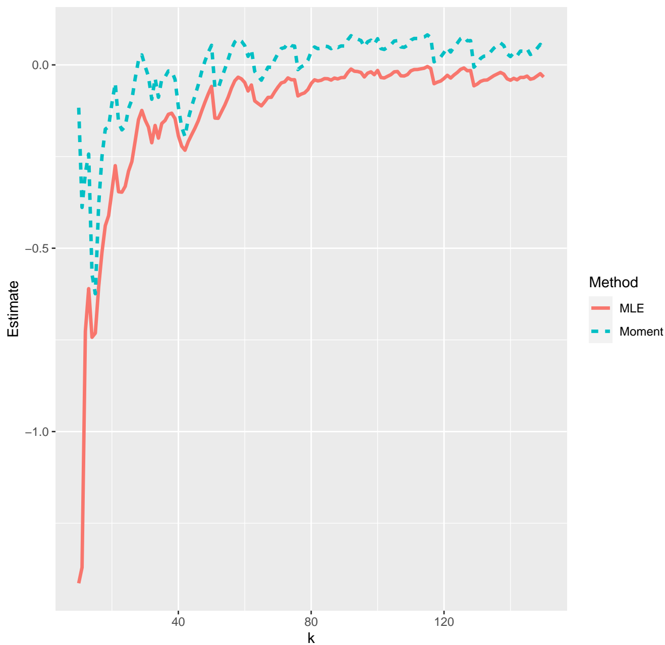
Estimates of extreme value index--29-09-2020
