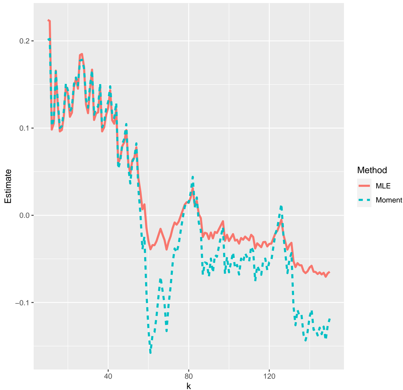
Estimates of extreme value index--27-12-2022
