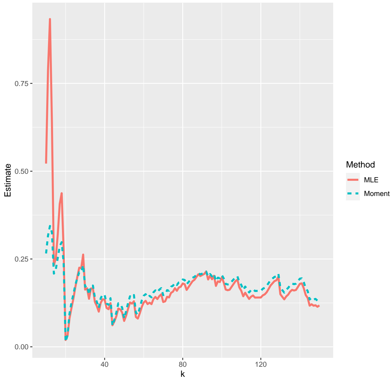
Estimates of extreme value index--27-09-2022
