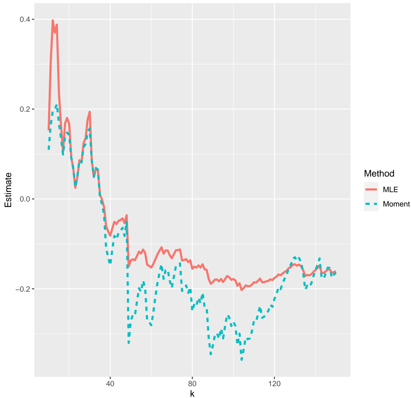
Estimates of extreme value index--27-04-2021
