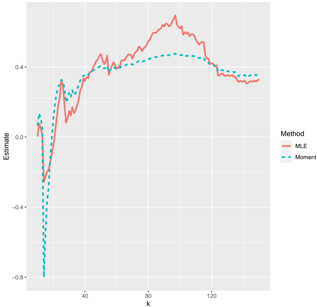
Estimates of extreme value index--26-10-2021
