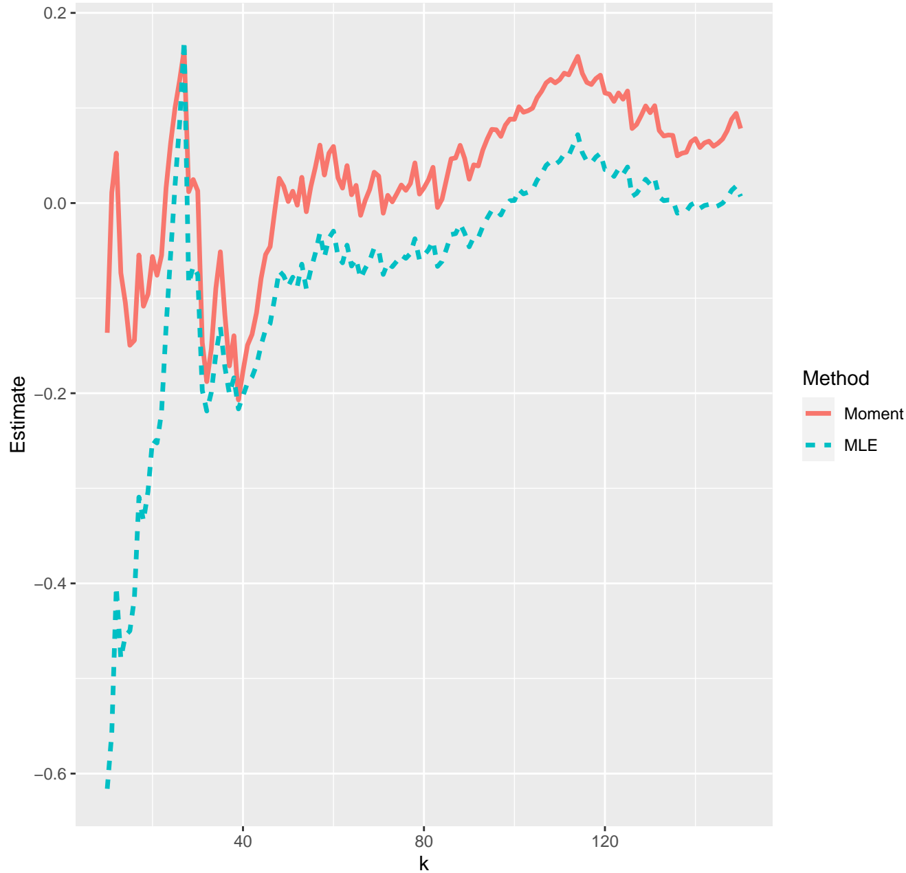
Estimates of extreme value index--26-04-2020
