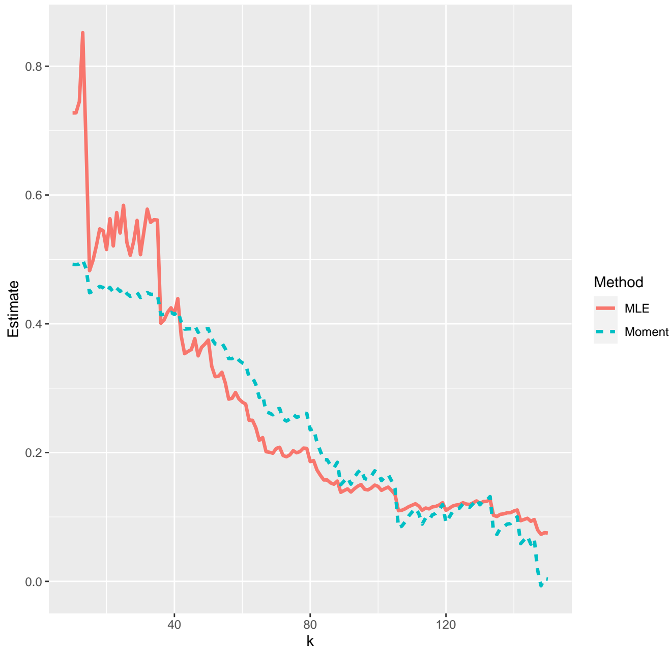
Estimates of extreme value index--25-11-2020
