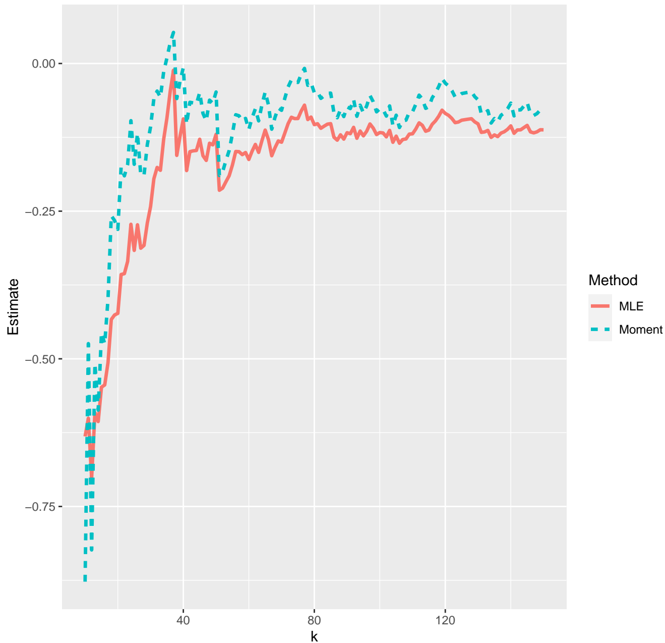
Estimates of extreme value index--25-10-2022
