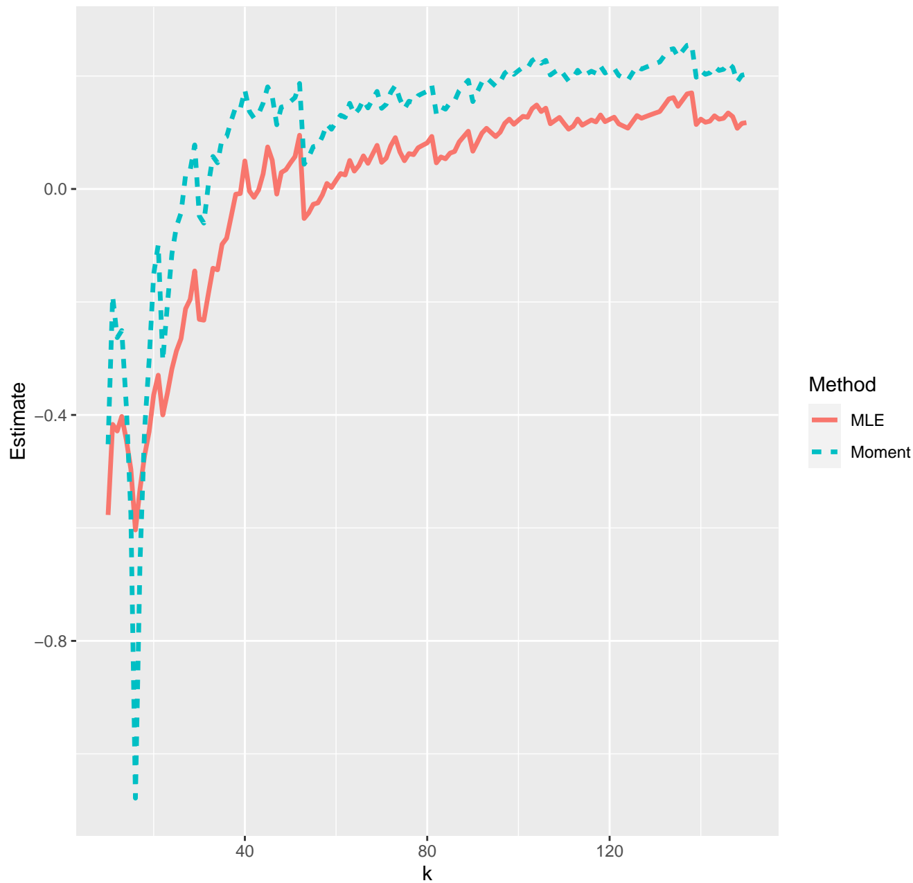
Estimates of extreme value index--25-08-2020
