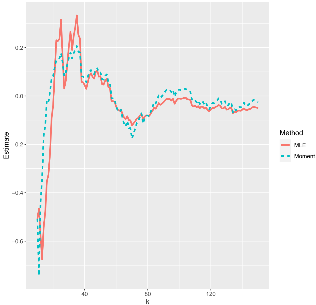
Estimates of extreme value index--25-05-2021
