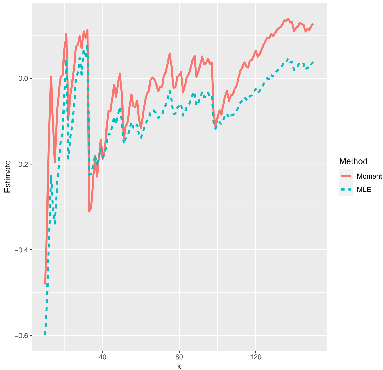
Estimates of extreme value index--25-05-2020
