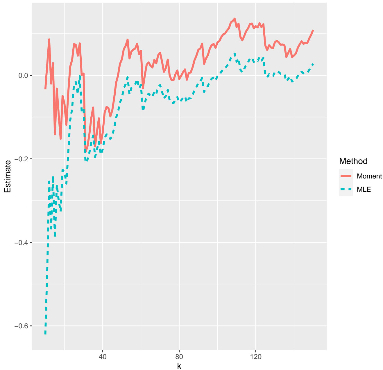
Estimates of extreme value index--25-04-2020
