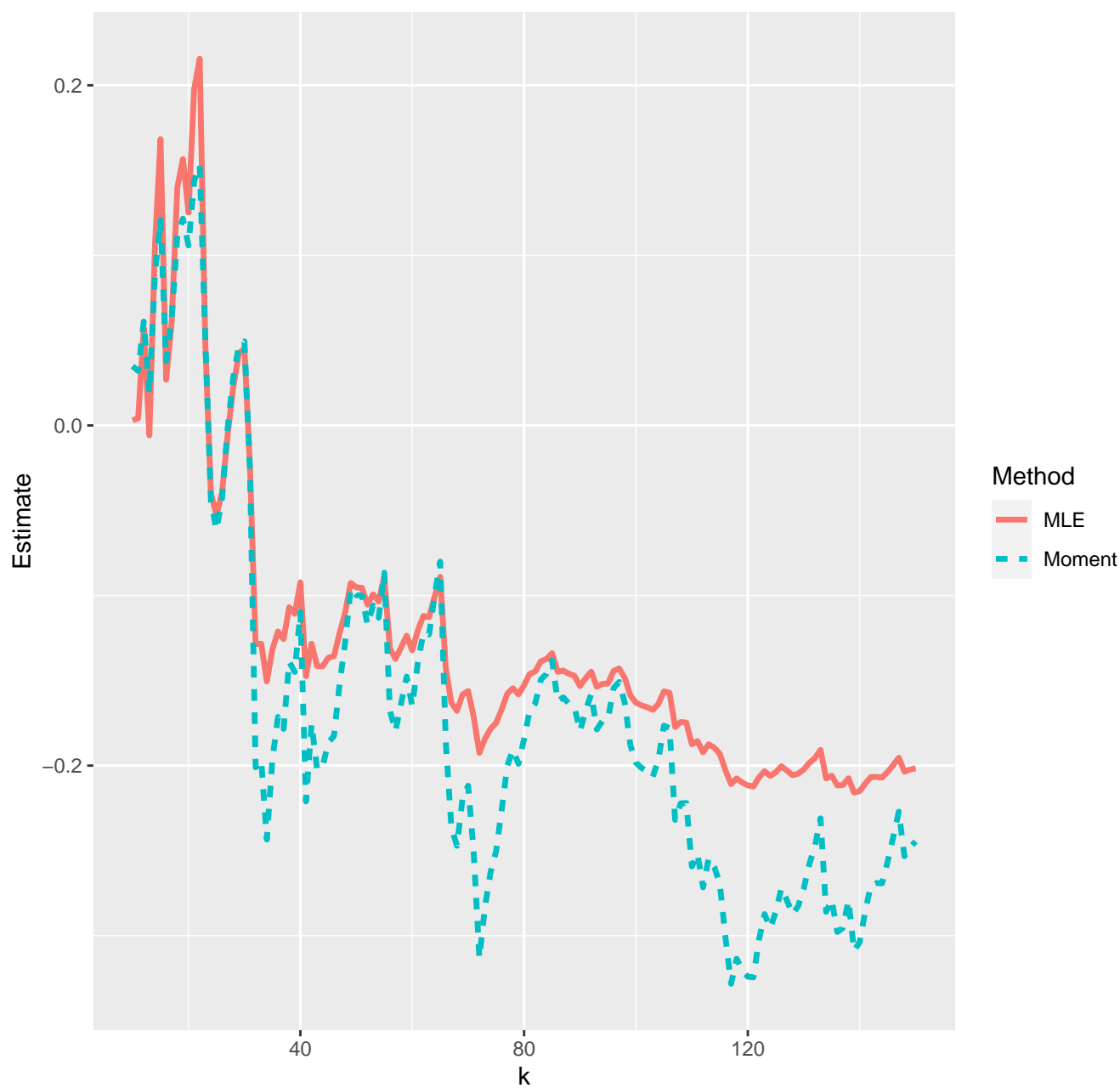
Estimates of extreme value index--25-01-2022
