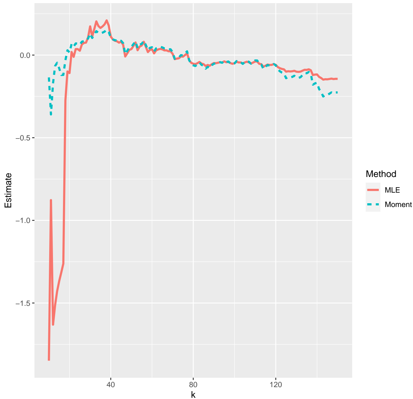
Estimates of extreme value index--23-11-2021
