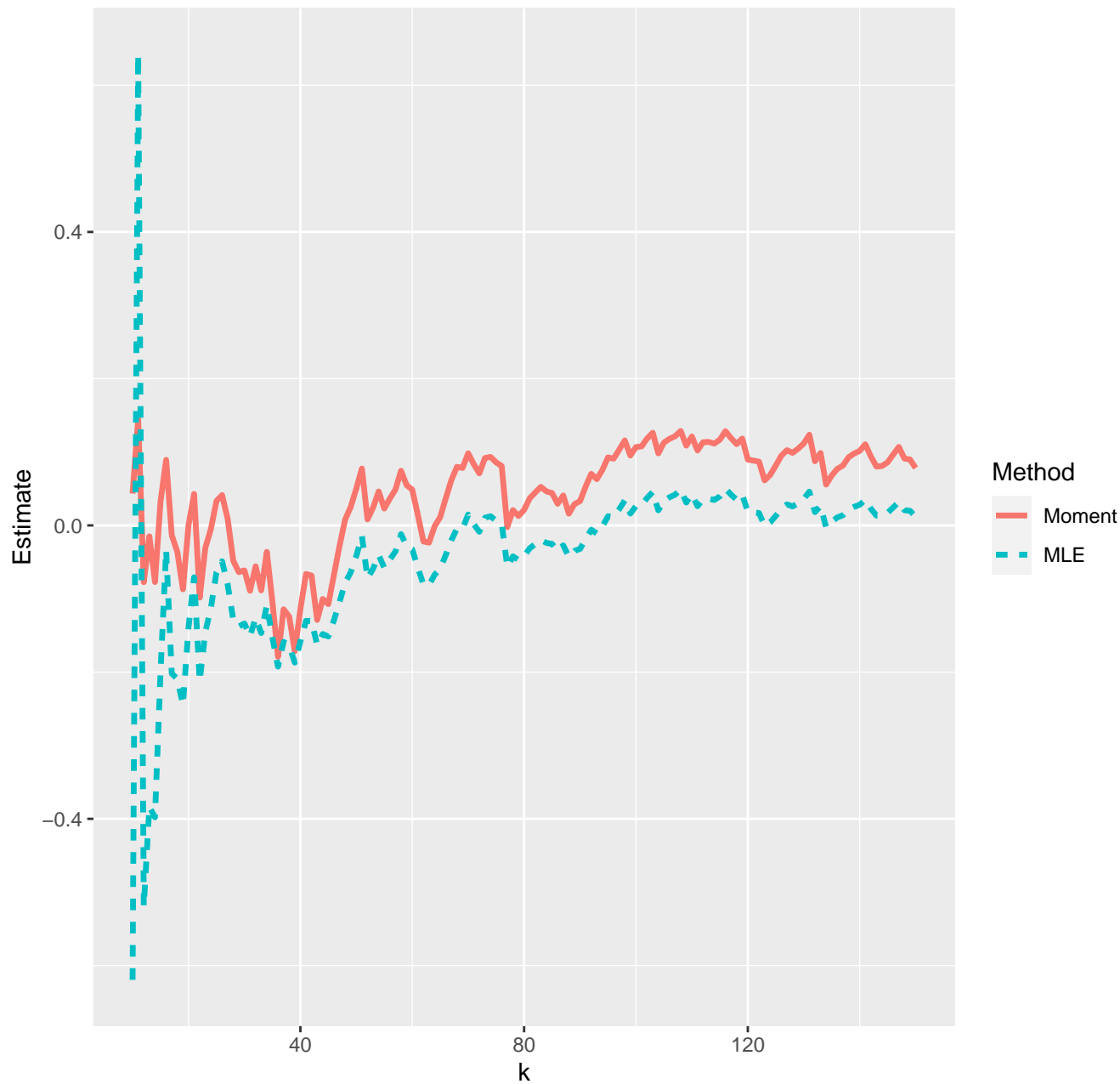
Estimates of extreme value index--23-04-2020
