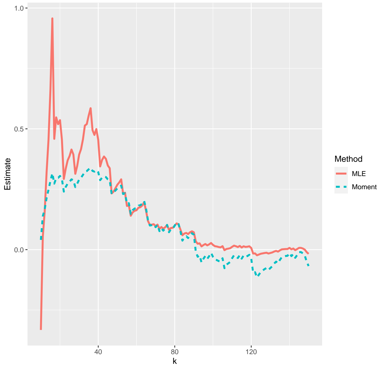
Estimates of extreme value index--23-03-2021
