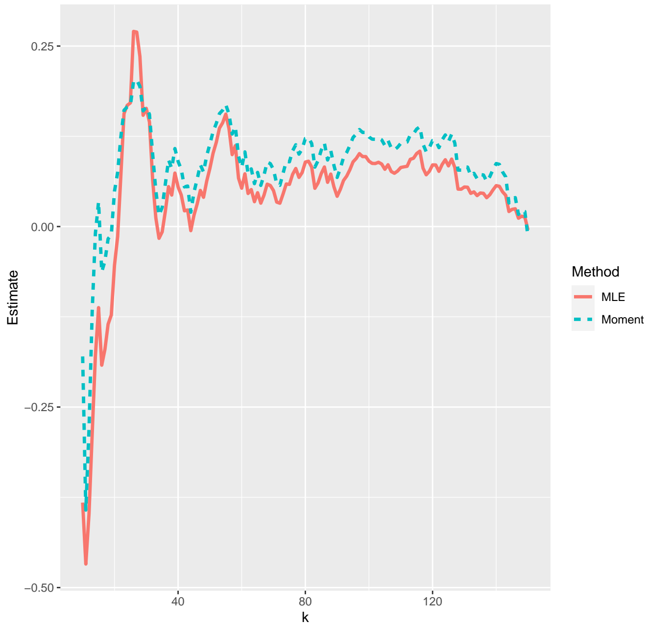
Estimates of extreme value index--23-02-2021
