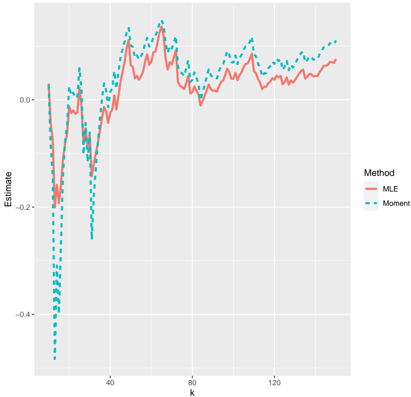
Estimates of extreme value index--22-12-2020
