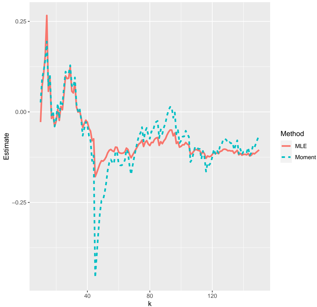
Estimates of extreme value index--22-06-2021
