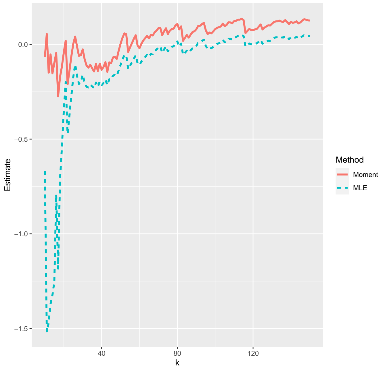
Estimates of extreme value index--22-04-2020
