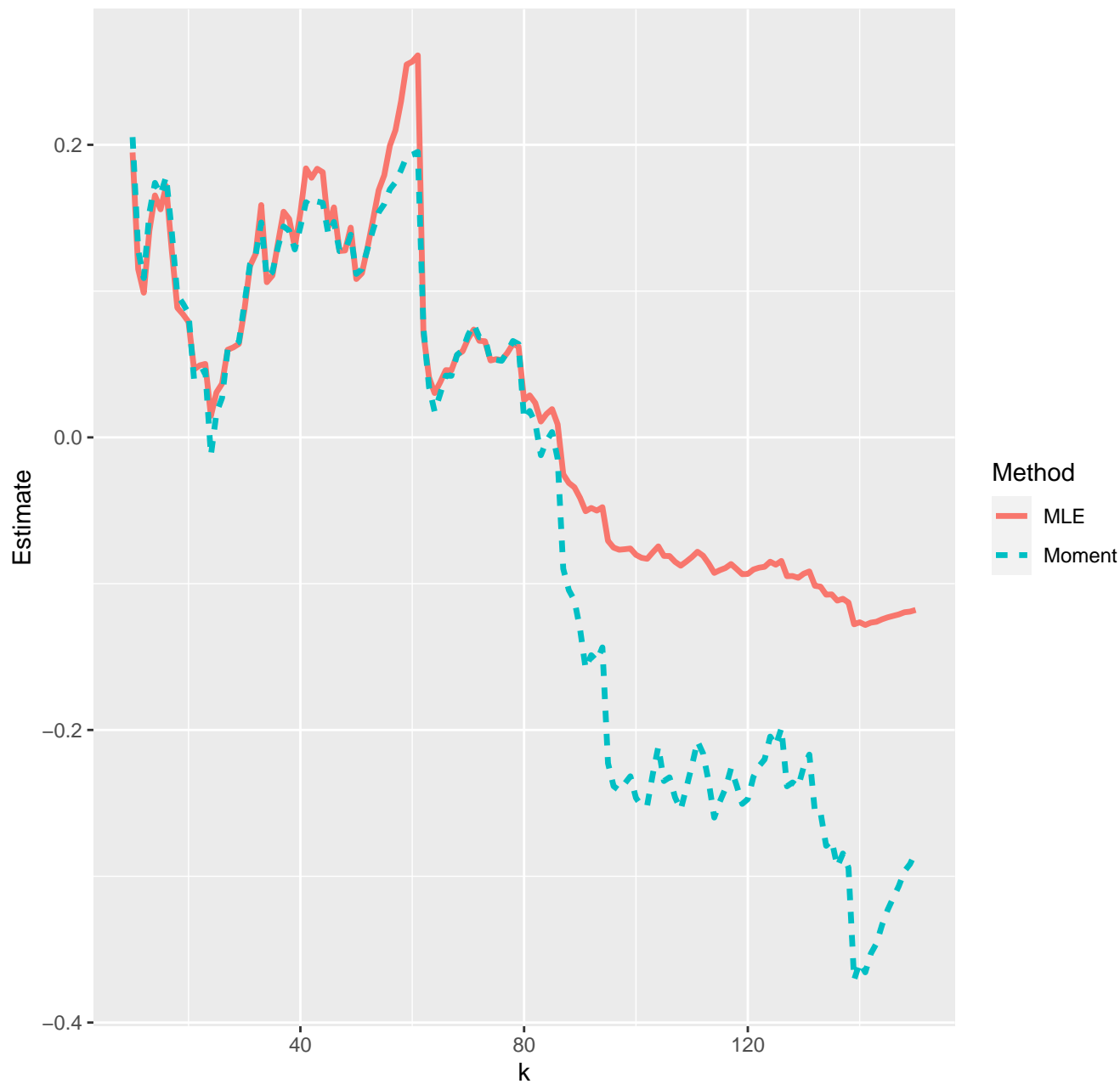
Estimates of extreme value index--22-03-2022
