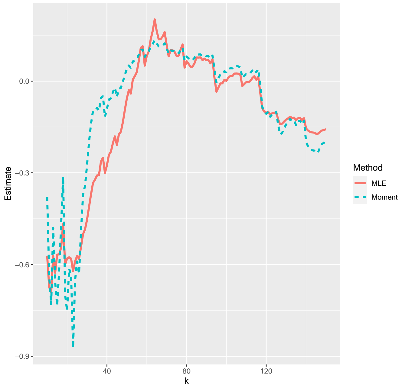
Estimates of extreme value index--22-02-2022
