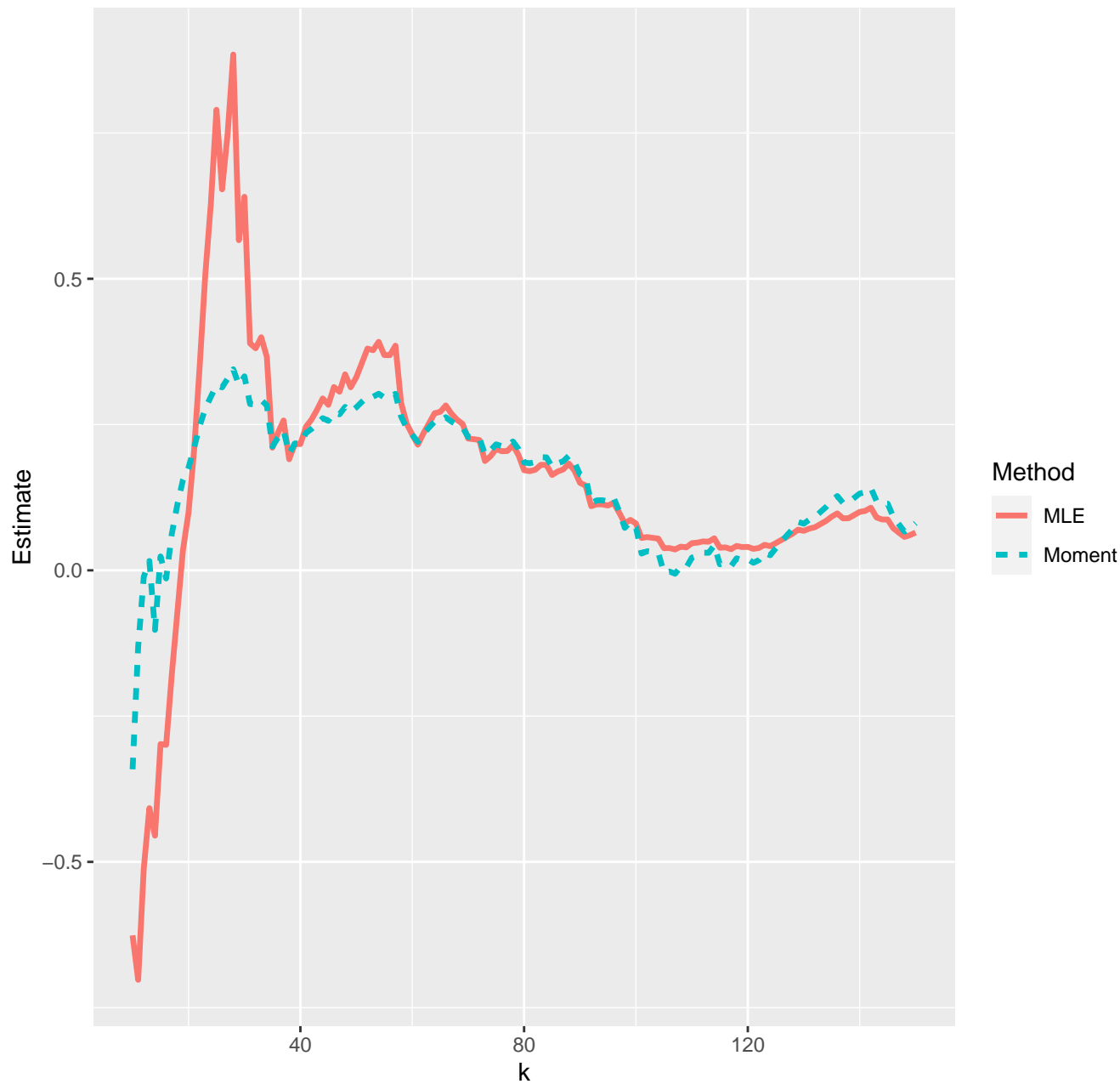
Estimates of extreme value index--21-09-2021
