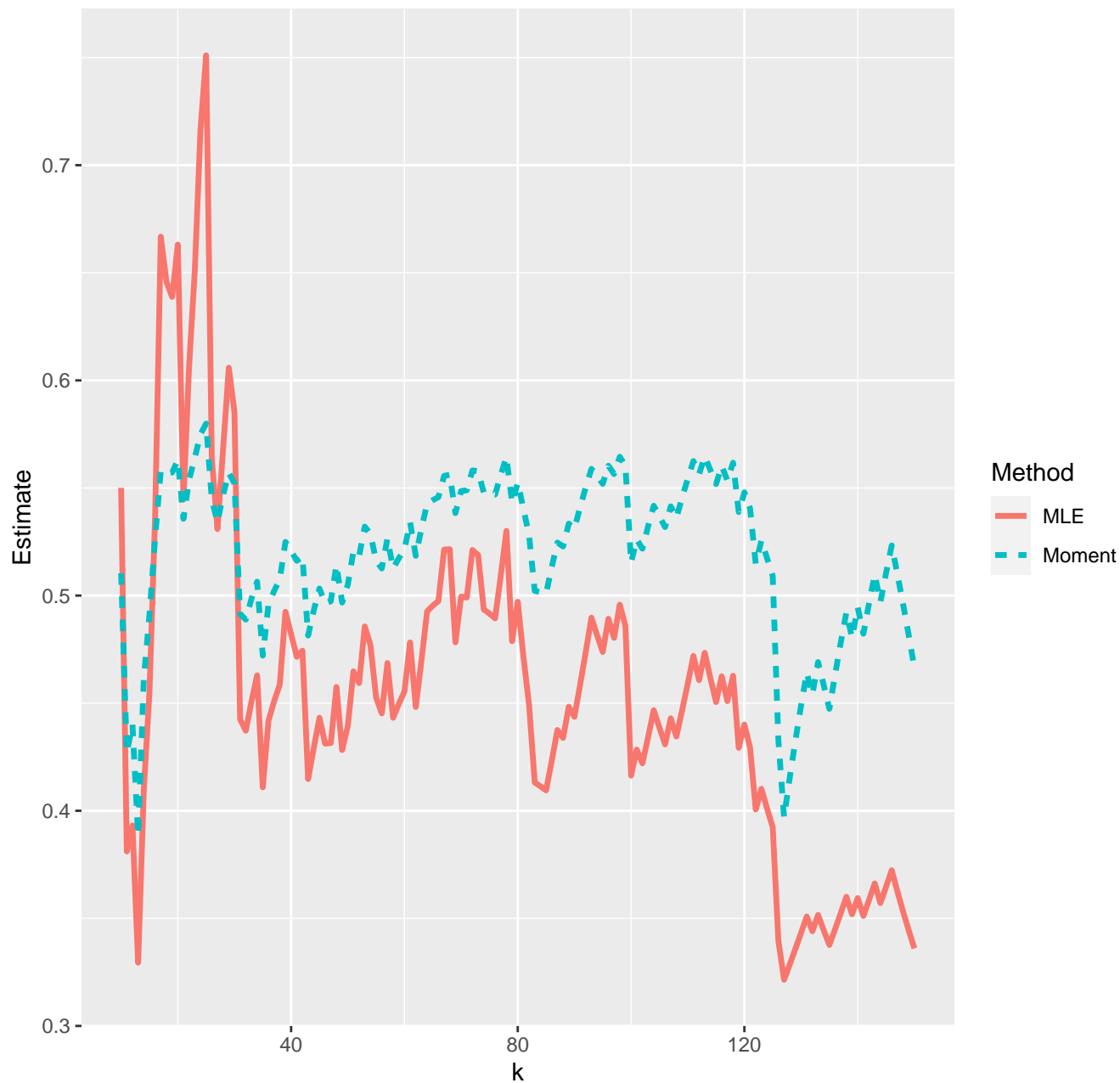
Estimates of extreme value index--21-07-2020
