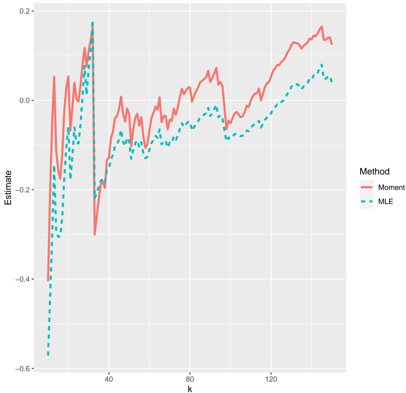
Estimates of extreme value index--21-05-2020
