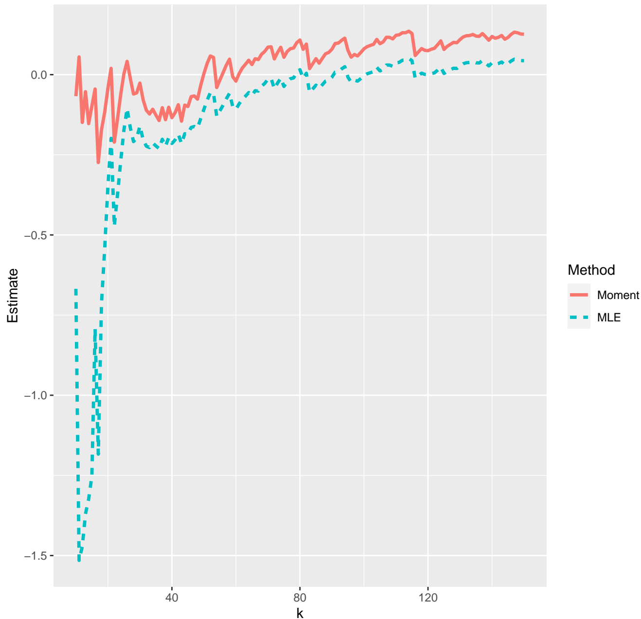
Estimates of extreme value index--21-04-2020
