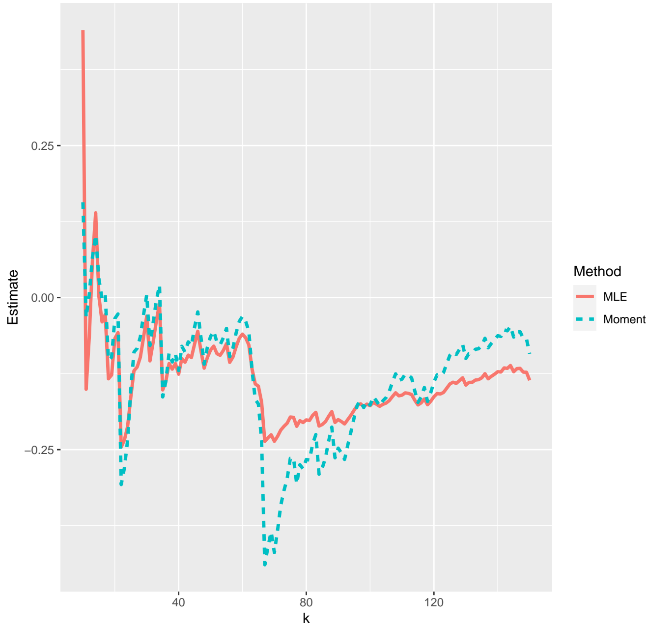
Estimates of extreme value index--20-04-2021
