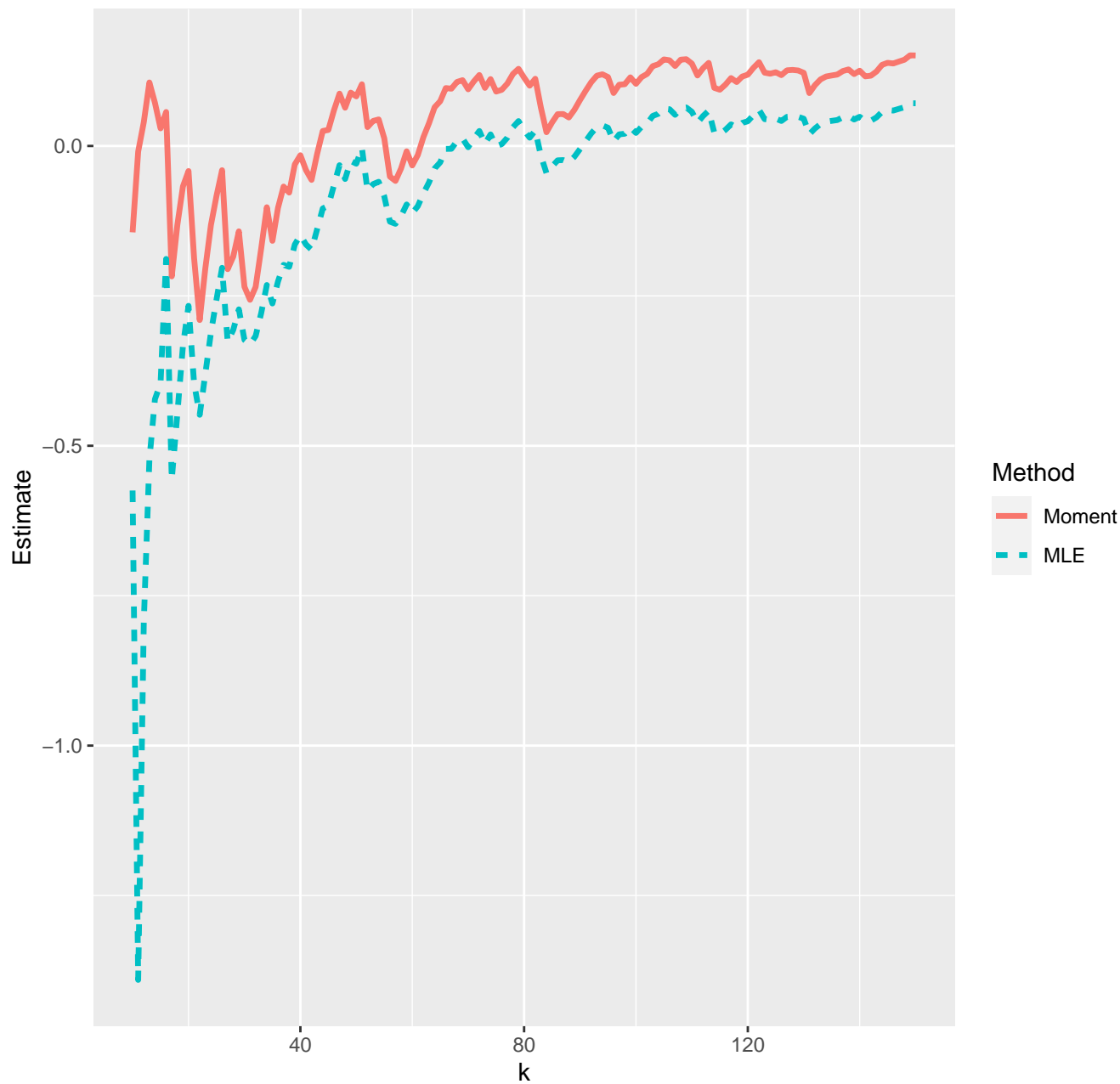
Estimates of extreme value index--19-04-2020
