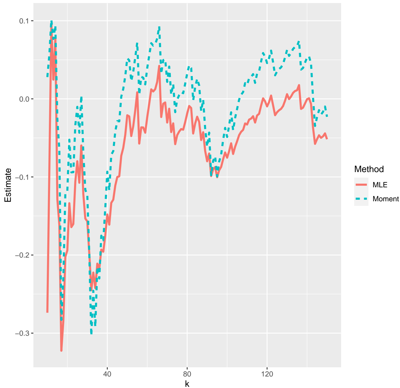
Estimates of extreme value index--19-01-2021
